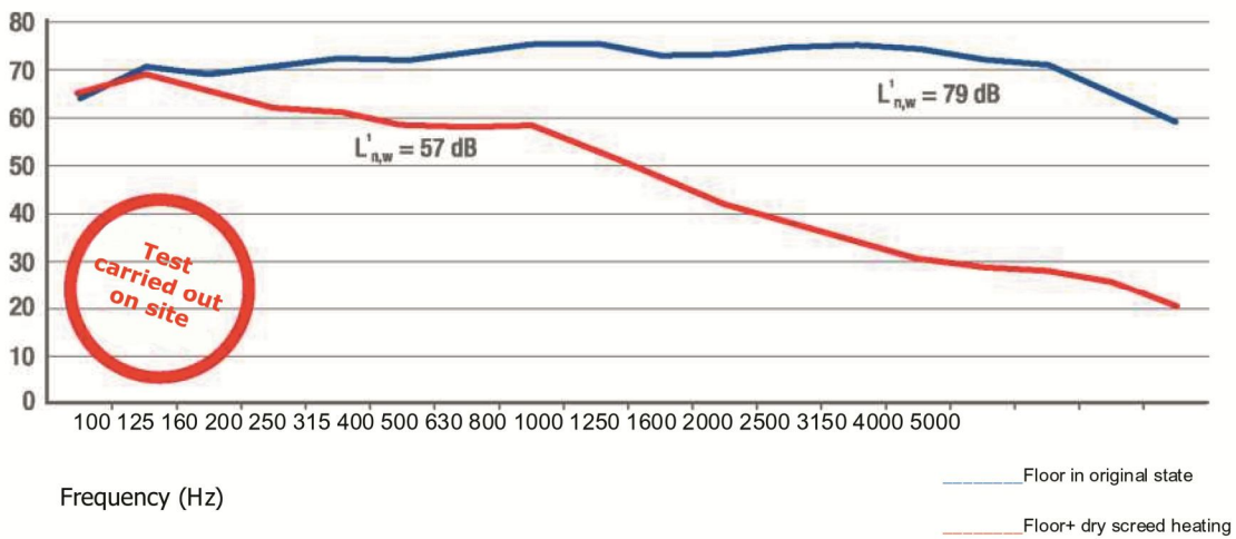
Comparative insulation test of rooms lagged with PV50
